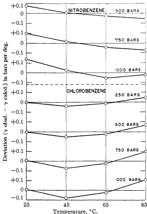
Fig. 4.—Deviations of the values of (\partial P/\partial T)_\gamma computed by the empirical equation (6) from the "observed" values.
